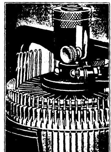
Fig. 41 Raising two needles at left
