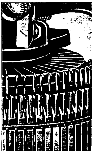
Fig. 23. Dial Set Too High for Knitting
