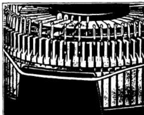
Fig. 32. Clasp spring out for removing needles.
