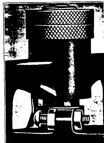
Fig. 31. Timing Dial, Let it Fast, Loosen Lock Nut at End
