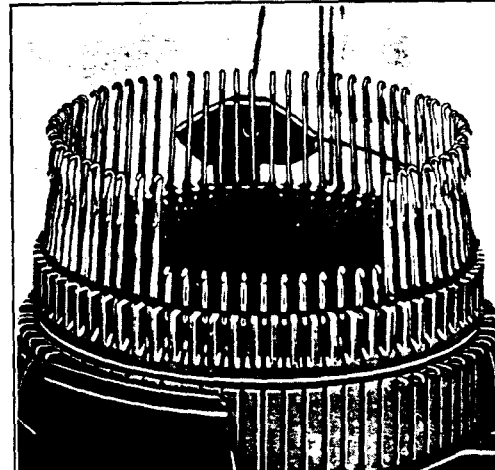
Fig. 43. Position of Needles Toe Half Knit
