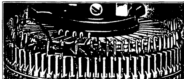
FIG. 21. Note Yarn Bunching Over Needles When Switch
