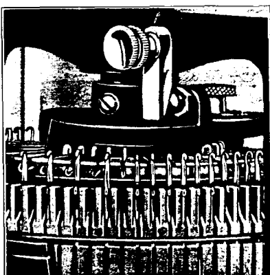
FIG. 19. MACHING Dial Slots With Control
