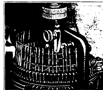
Fig. 34. Back Needles Raised for Making Heel
