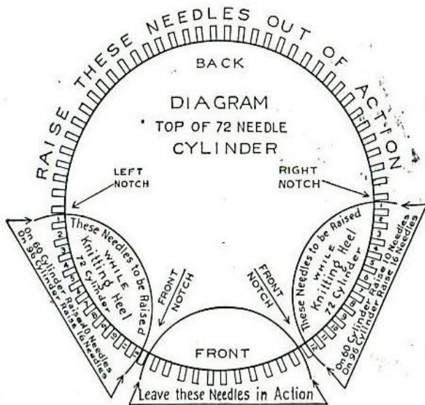
Figure 33. Diagram of Cylinder Showing How to Knit Heel and Toe
