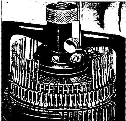
FIG. 39. POSITION OF NEEDLES HEEL Half knit
